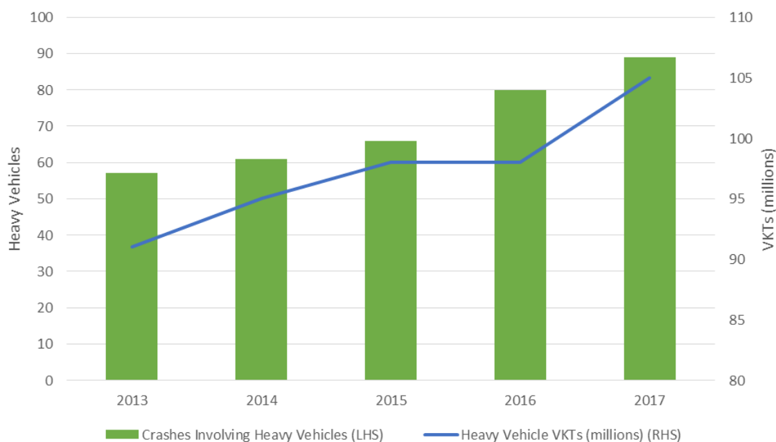
Figure 36. Northland heavy vehicle crashes compared with heavy vehicle travel - 2013 to 2017
