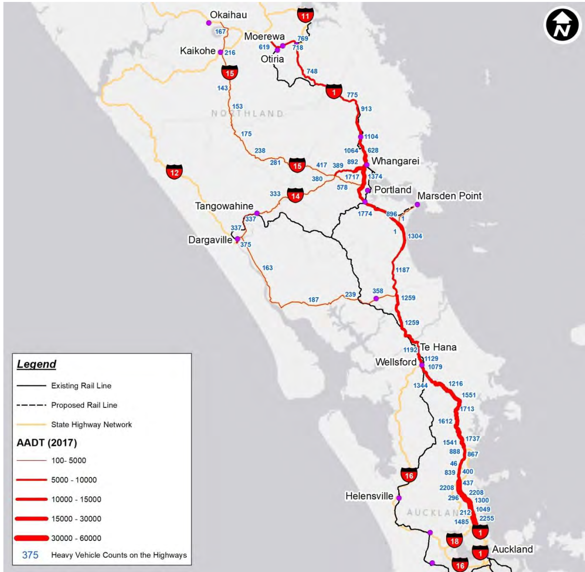
Figure 34. Annual Average Daily Travel, with Heavy Vehicle counts – State Highway 1
