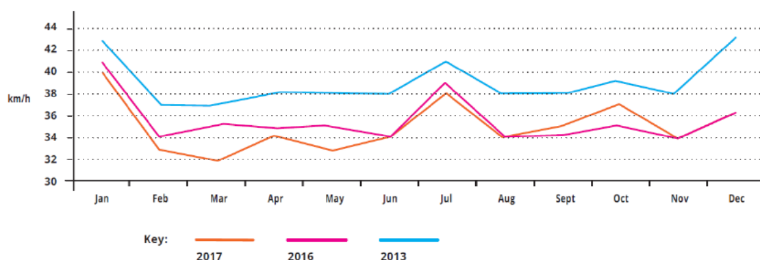
Figure 51. Auckland arterial road network - morning peak average speed, 2013-2017
