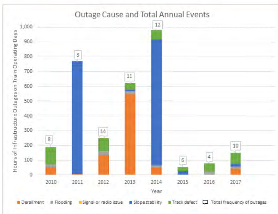
Figure 32: North Auckland Line Infrastructure Outages 2010-17
