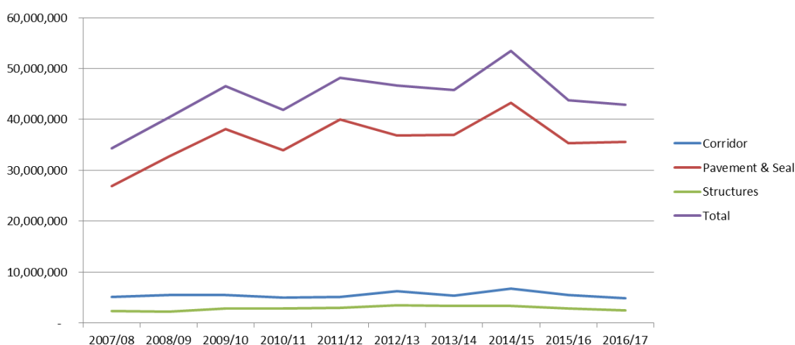
Figure 17. Northland State highway maintenance expenditure 2007-2016
