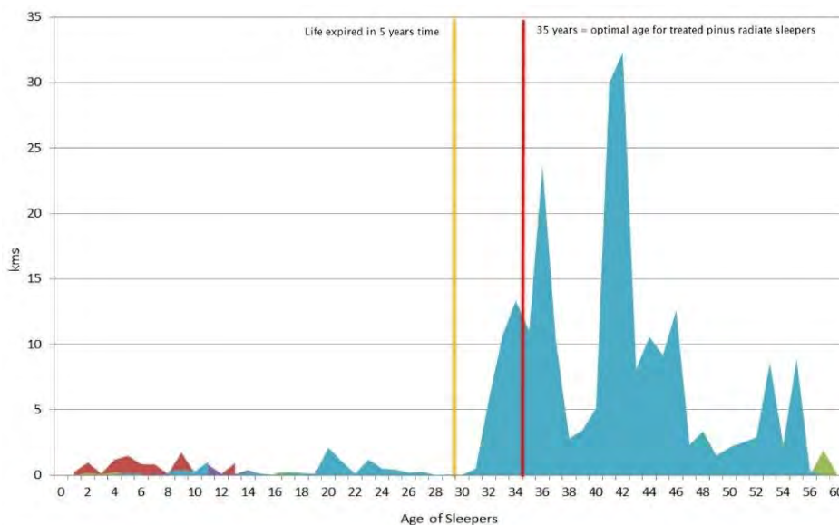
Figure 15. Sleeper Age Profile
