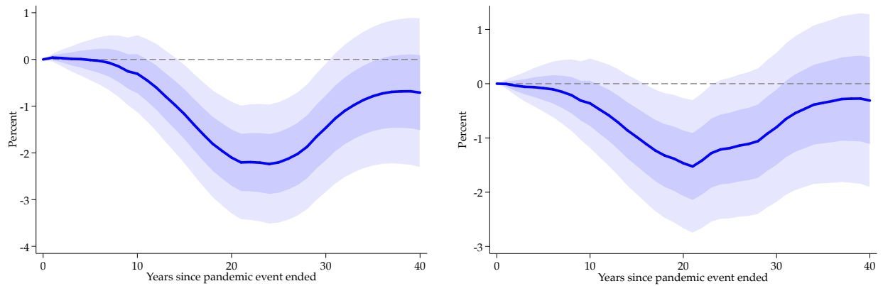
Figure 7: Response of the European real natural rate of interest following pandemics, (a) excluding the Black Death (b) excluding the 1918 Spanish Flu
